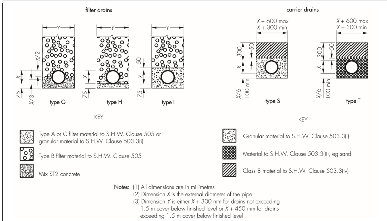
Figure 3 Installation details
