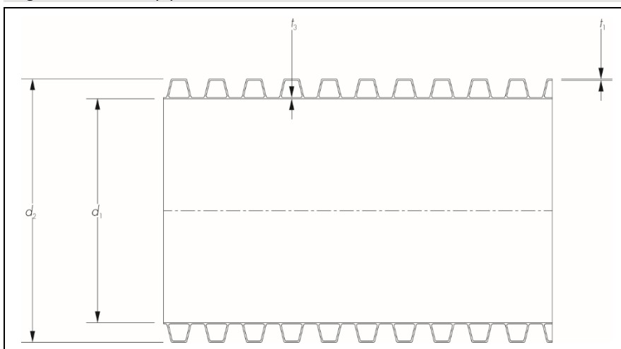
Figure 1 Twinwall pipe dimensions
